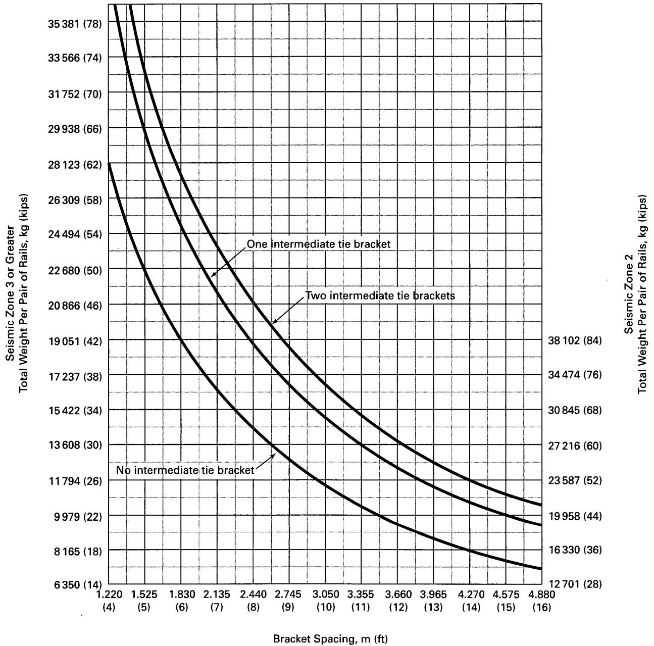
Fig. 8.4.8.2-6 33.5 kg/m (22.5 lb/ft) Guide-Rail Bracket Spacing
