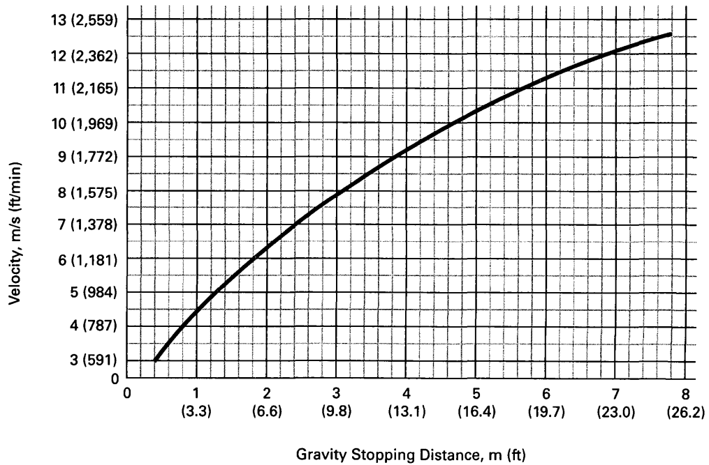
Fig. 8.2.4 Gravity Stopping Distances
