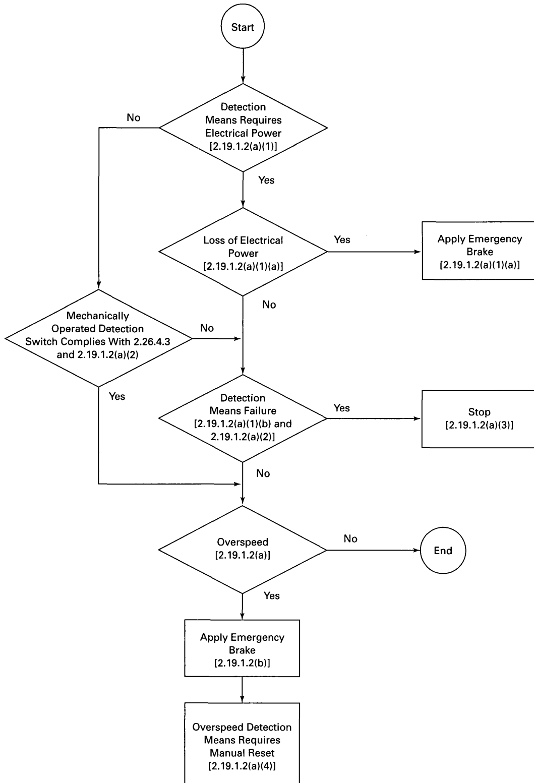
Fig. F-1 Ascending Car Overspeed Protection (2.19.1)
