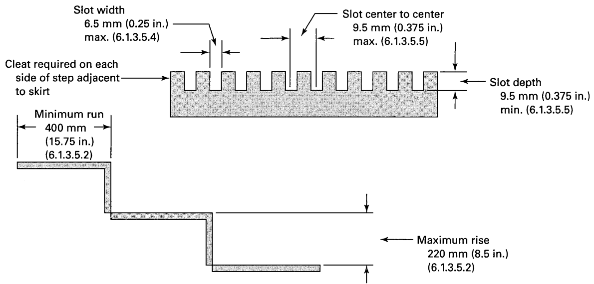
Fig. I-7 Escalator Step Tread
