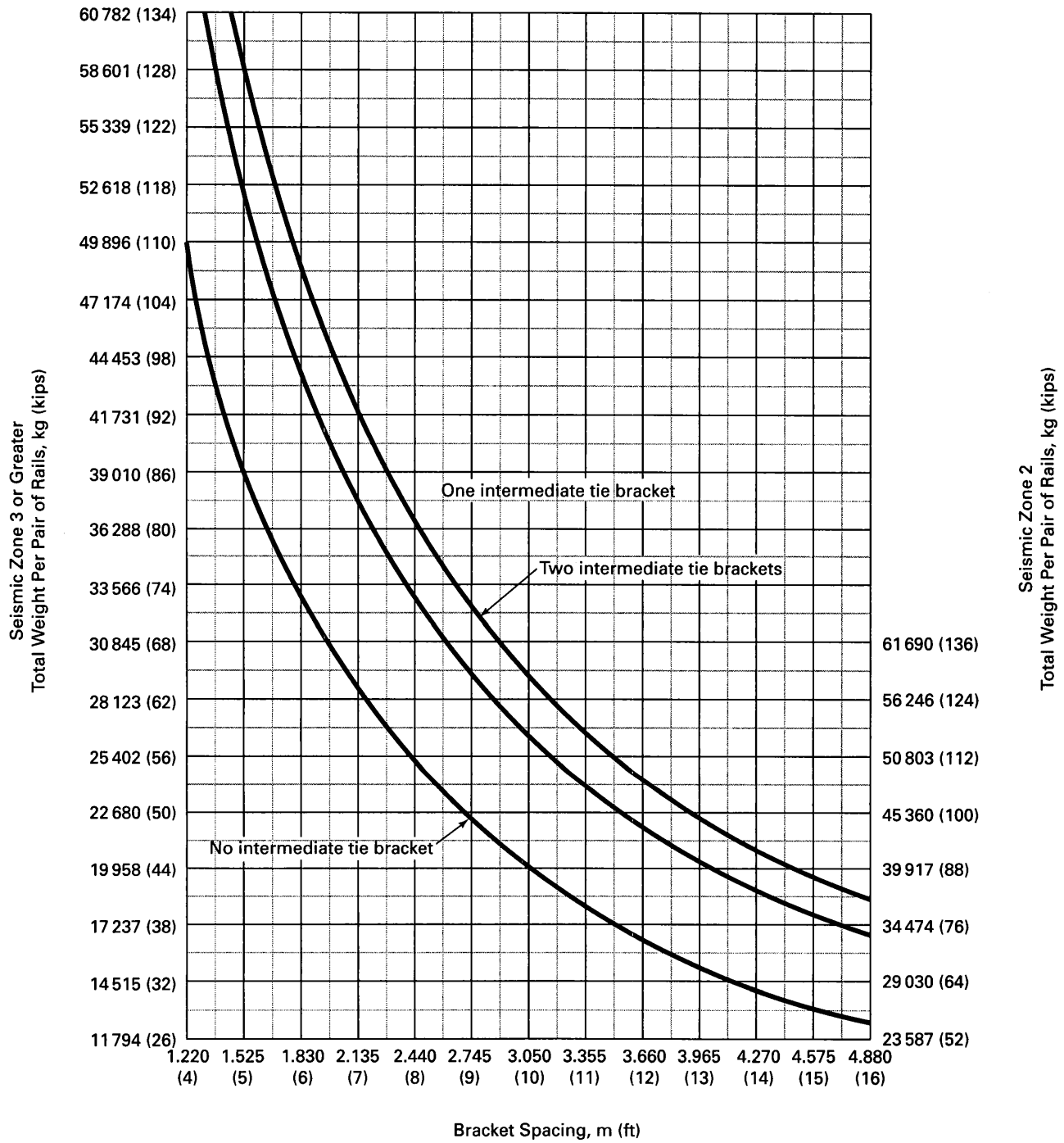
Fig. 8.4.8.2-7 44.5 kg/m (30 lb/ft) Guide-Rail Bracket Spacing
