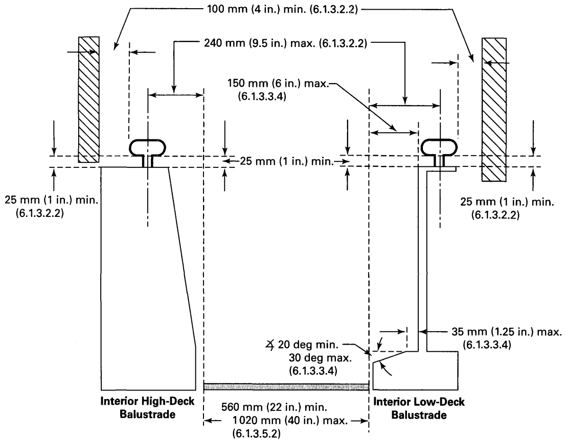
Fig. I-1 Relationship of Escalator Parts
