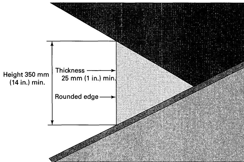
Fig. I-5 Ceiling or Soffit Guard (6.1.3.3.9)
