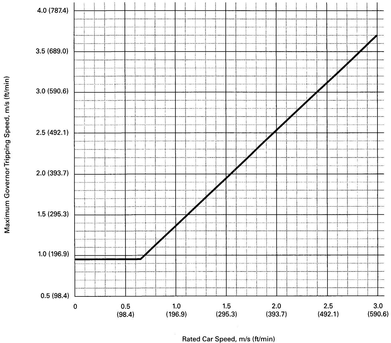
Fig. 8.2.5 Maximum Governor Tripping Speeds
