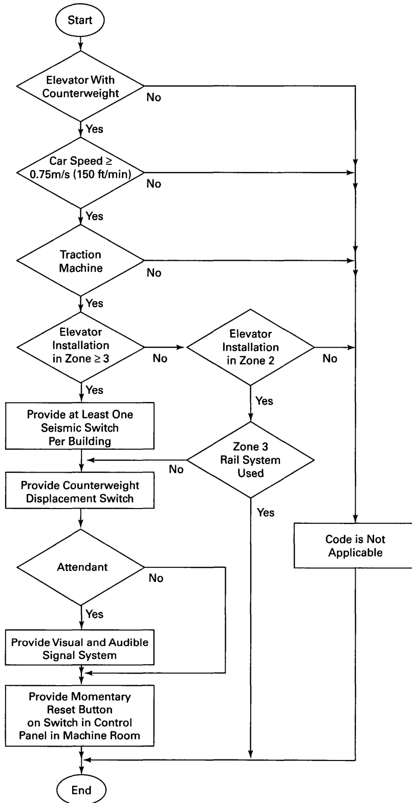
Fig. 8.4.10.1.1 Earthquake Elevator Equipment Requirements Diagrammatic Representation
