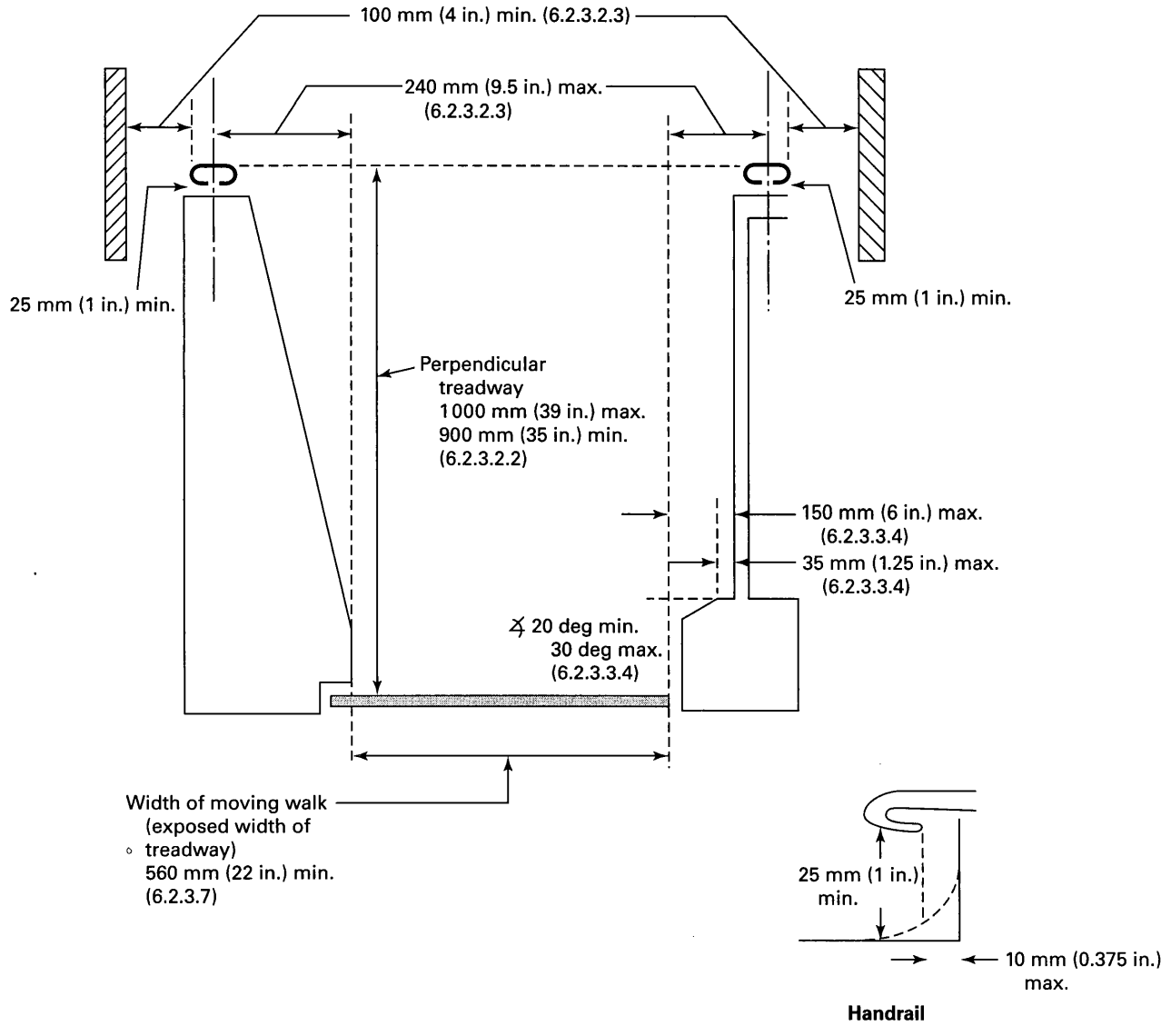
Fig. I-9 Moving Walk Geometry
