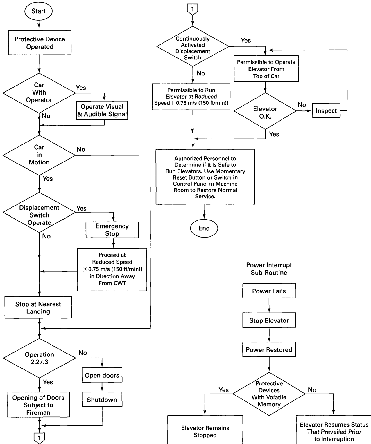
Fig. 8.4.10.1.3 Earthquake Emergency Operation Diagrammatic Representation
