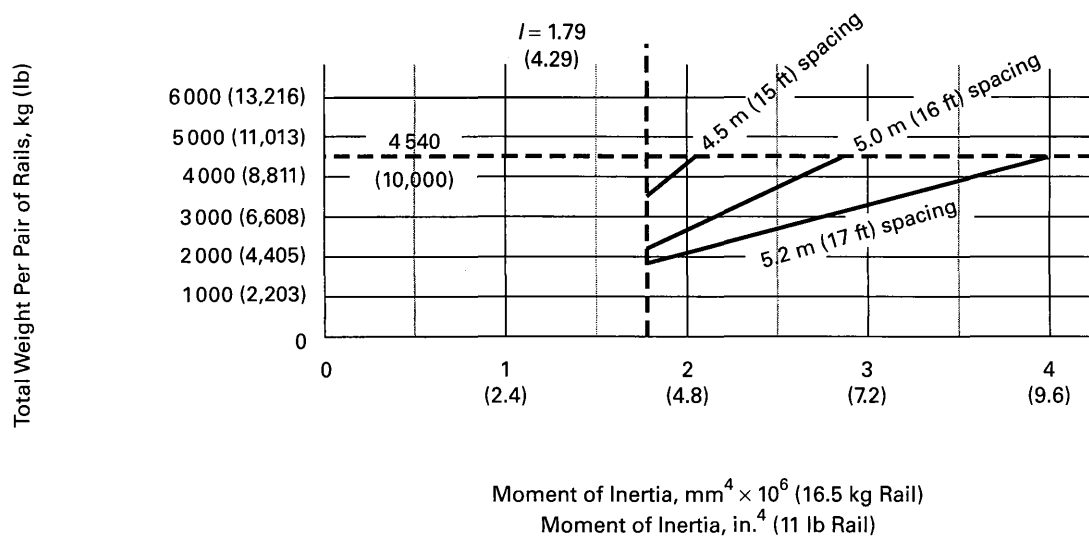
Fig. 2.23.4.1-2 Minimum Moment of Inertia About x-x Axis for a Single Guide Rail With Its Reinforcement
