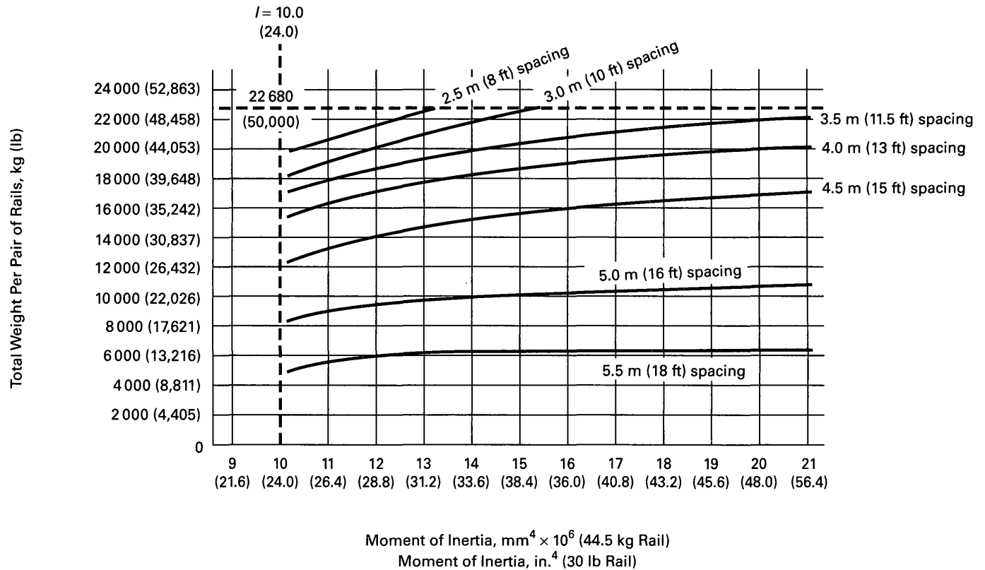
Fig. 2.23.4.1-2 Minimum Moment of Inertia About x-x Axis for a Single Guide Rail With Its Reinforcement (Cont'd)
