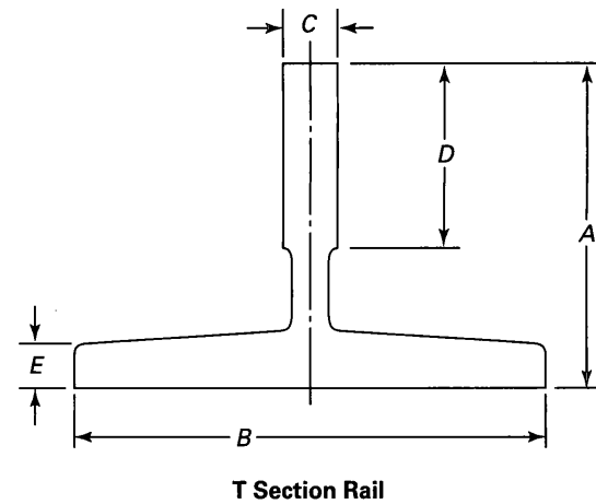
Fig. 2.23.3 Elevator Guide Rails
