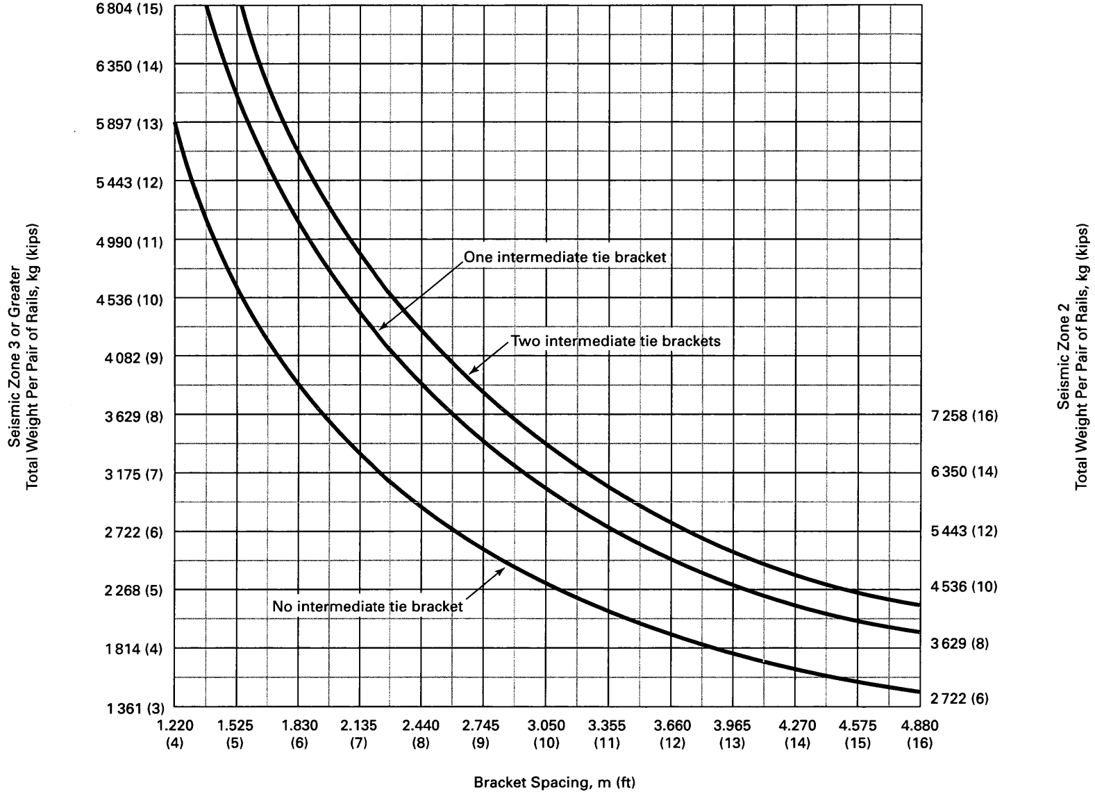
Fig. 8.4.8.2-1 12 kg/m (8 lb/ft) Guide-Rail Bracket Spacing
