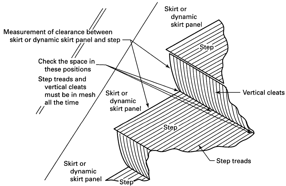
Fig. I-8 Cleated Riser (6.1.3.5.3)
