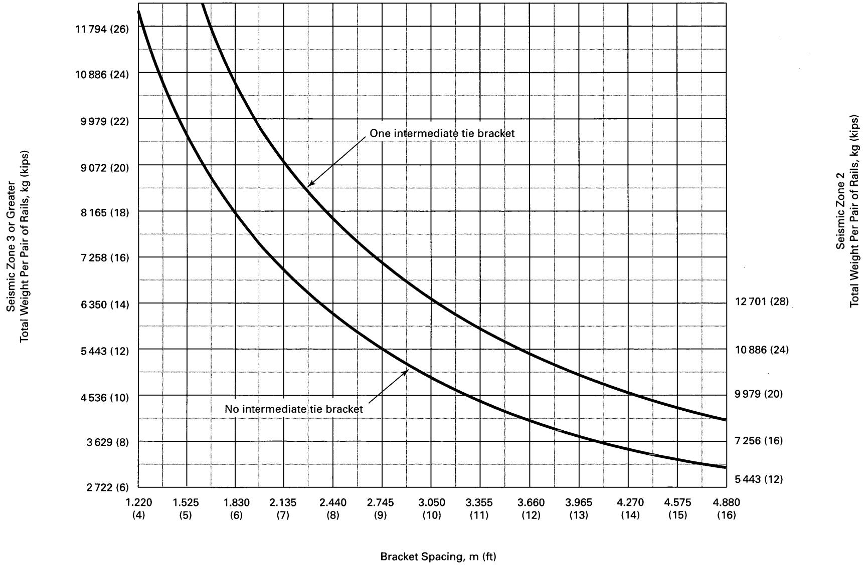
Fig. 8.4.8.2-2 16.5 kg/m (11 lb/ft) Guide-Rail Bracket Spacing
