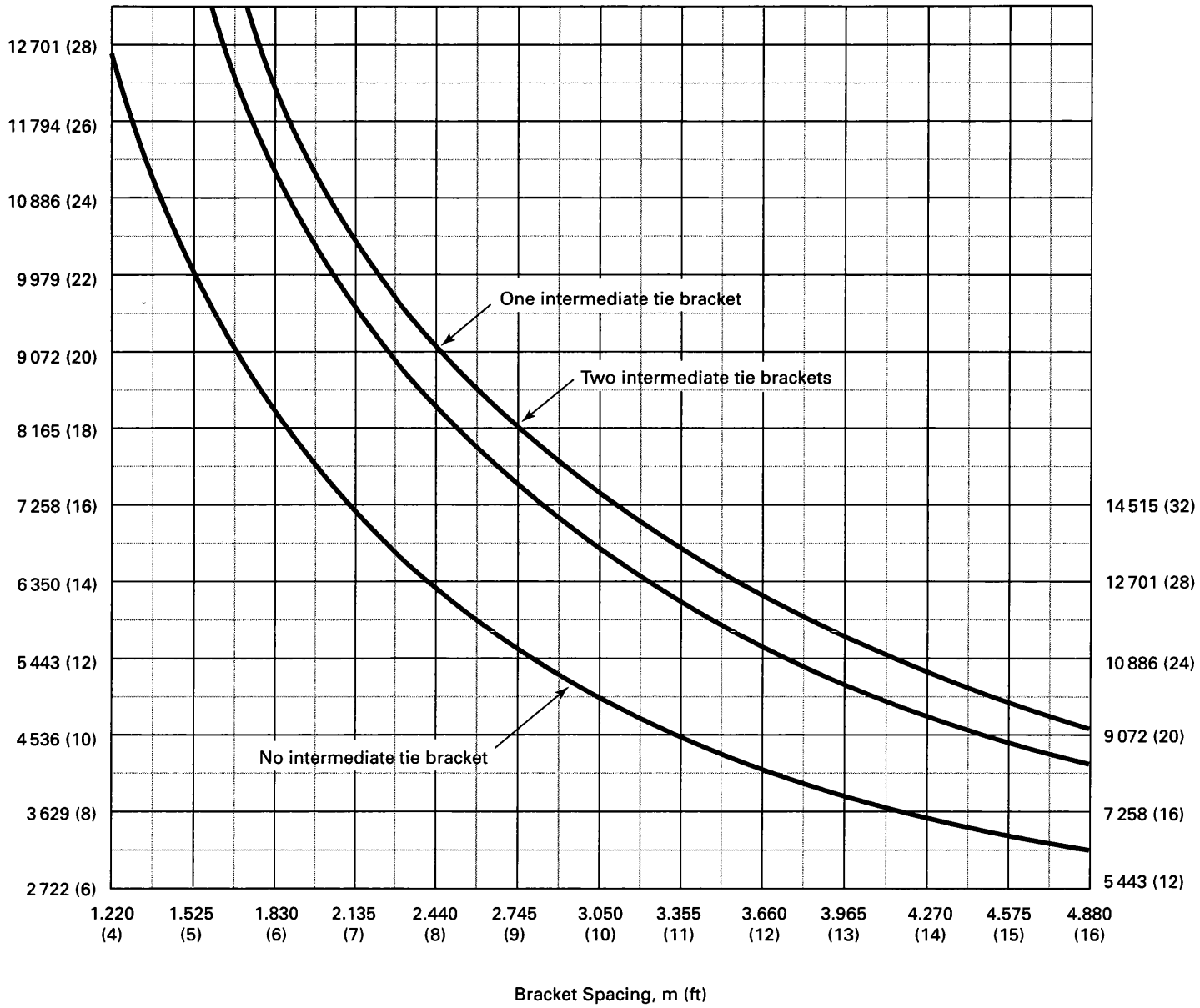
Fig. 8.4.8.2-3 18 kg/m (12 lb/ft) Guide-Rail Bracket Spacing
