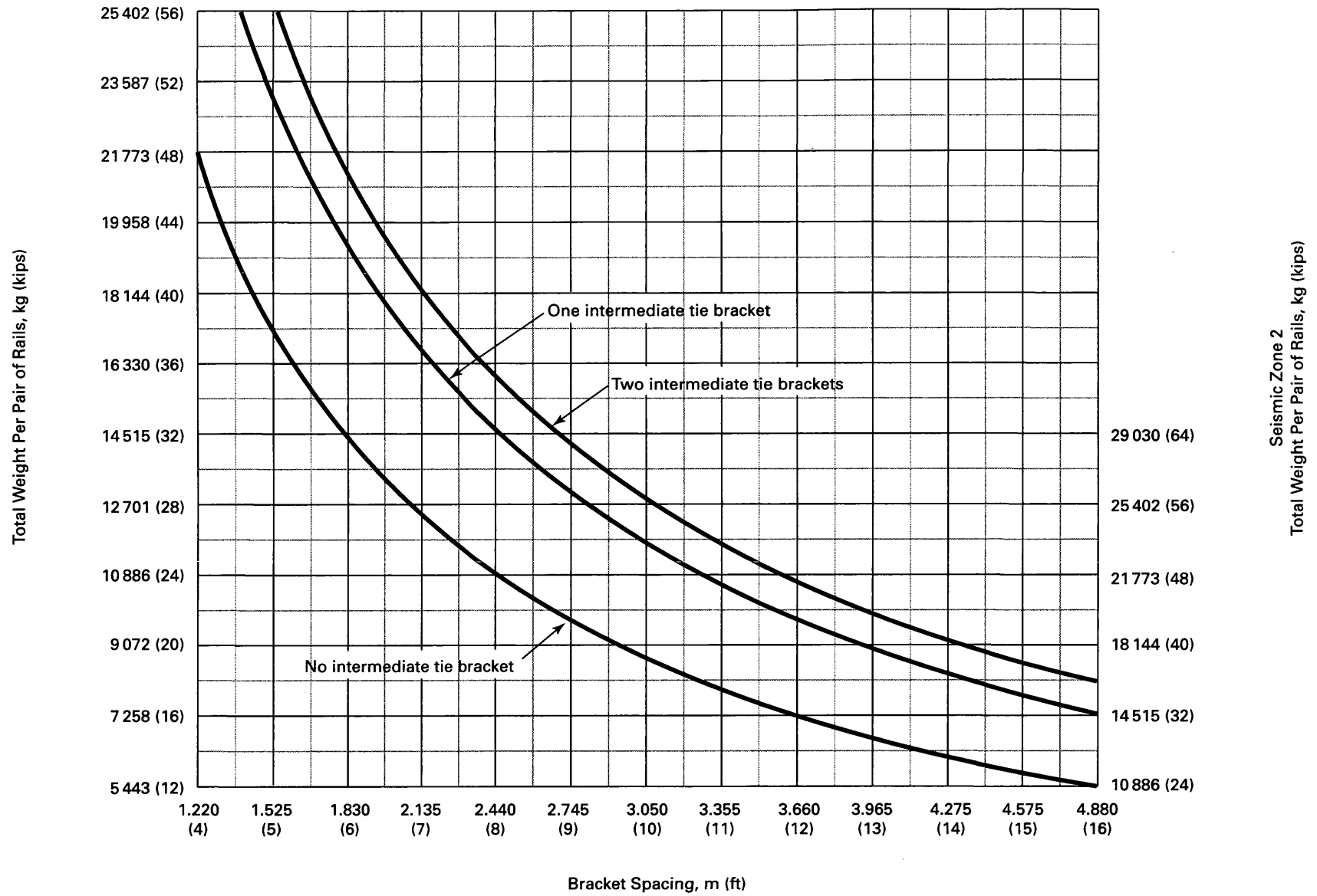
FIG. 8.4.8.2-5 27.5 kg/m (18.5 lb/ft) Guide-Rail Bracket Spacing
