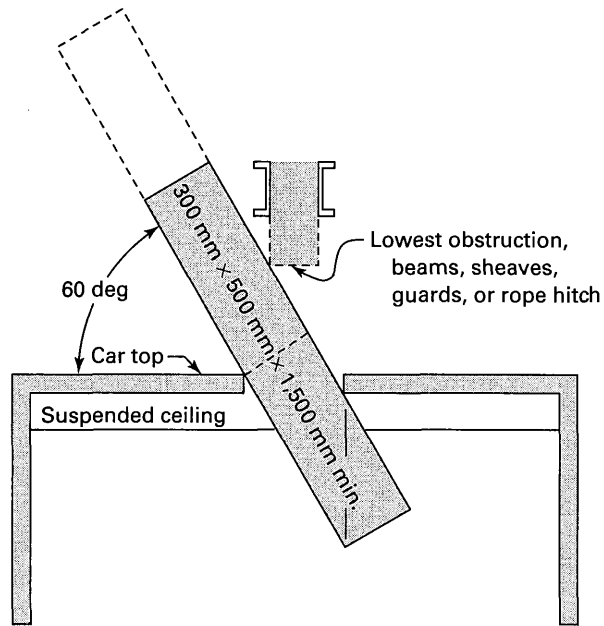
Fig. C-1 Parallelepiped Volume Orientations [2.14.1.5.1(b)(2)]
