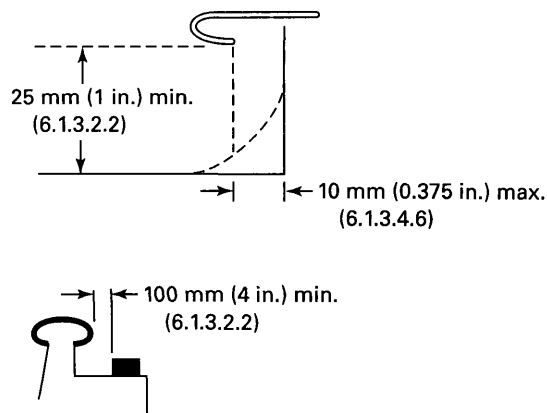
Fig. I-2 Handrail
