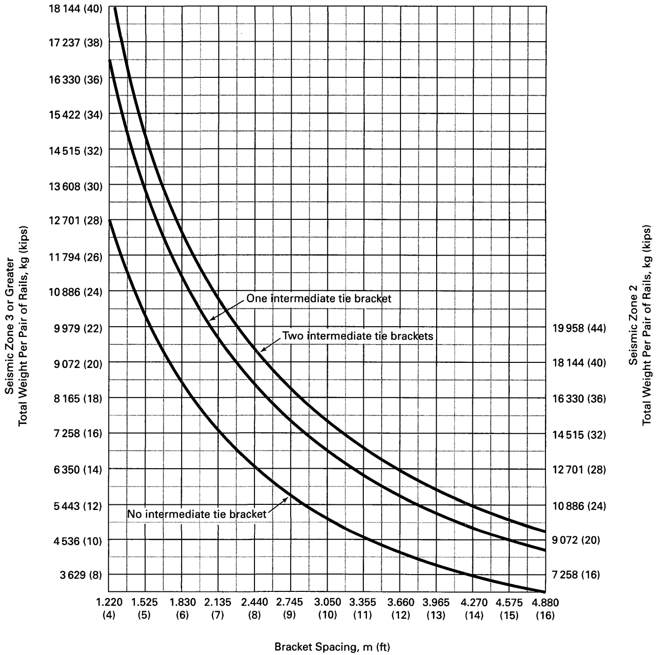
Fig. 8.4.8.2-4 22.5 kg/m (15 lb/ft) Guide-Rail Bracket Spacing
